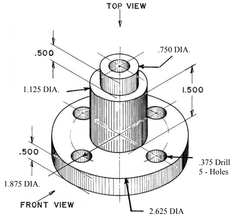
IN-26 - Shaft Support
