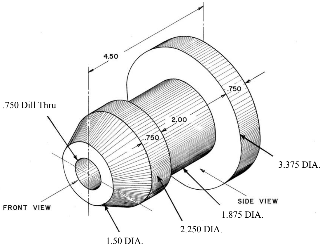
IN-29 Cone Support
