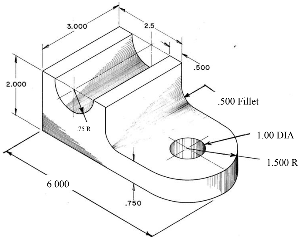
IN-22 Shaft Support
