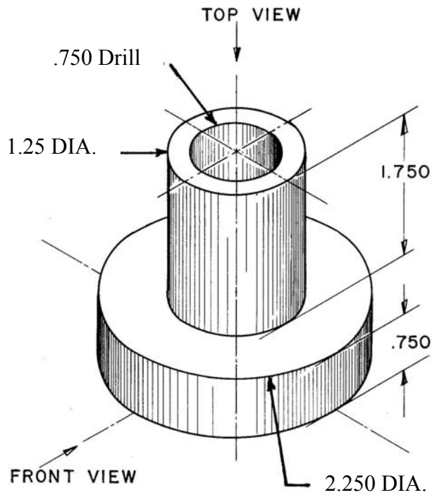
IN-25 - Flanged Bushing
