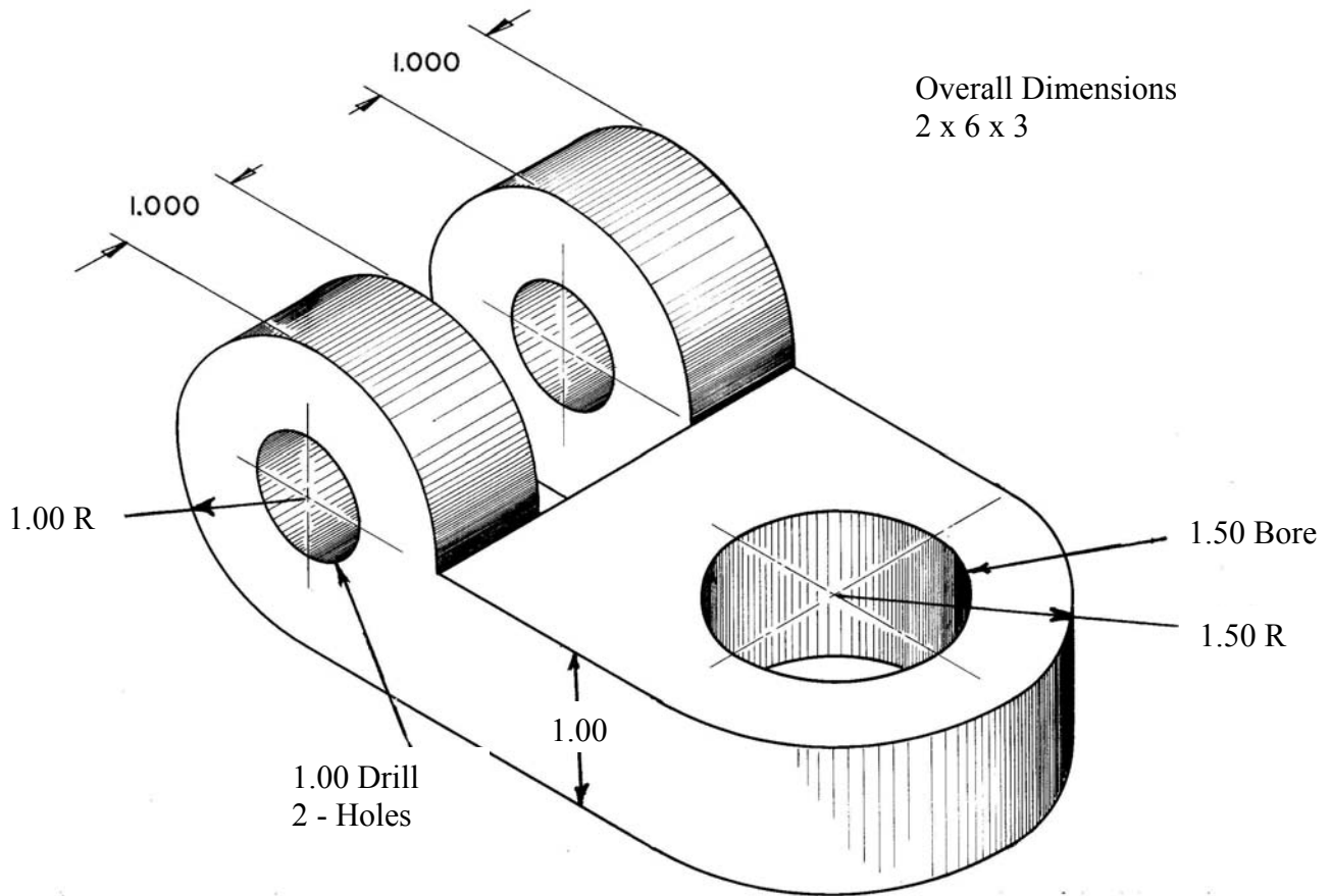
IN-24 - Reverse Link
