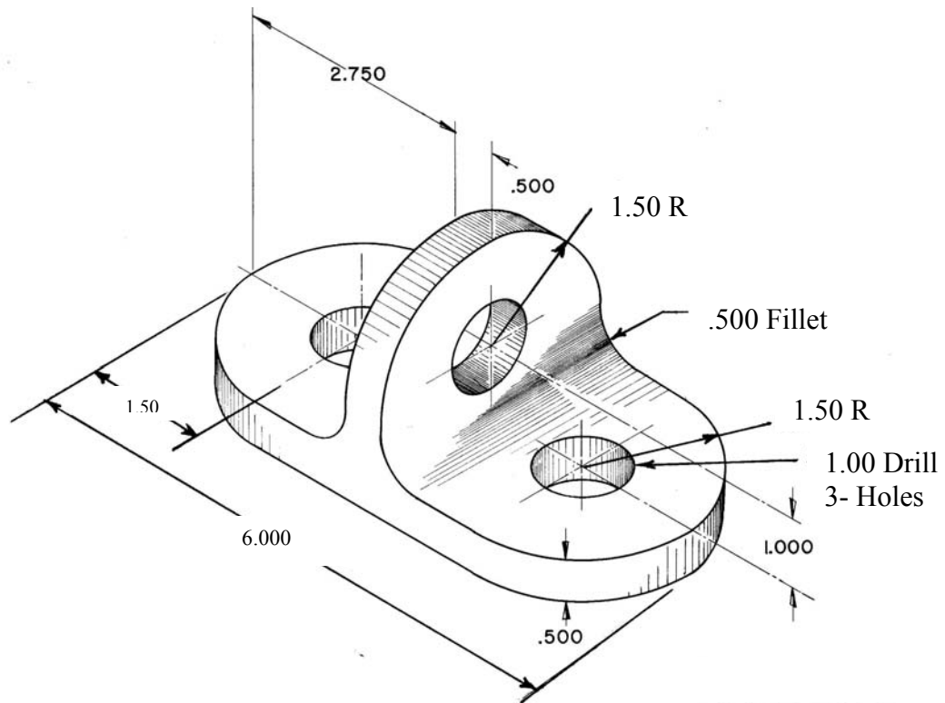
IN-23 Bracket
