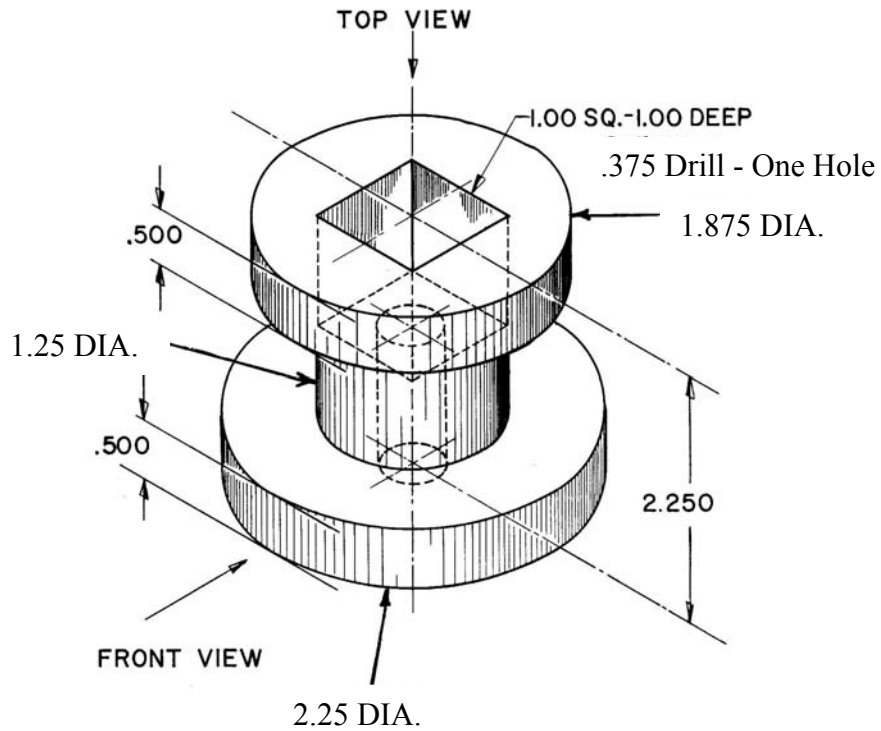
IN-27 Special Spacer
