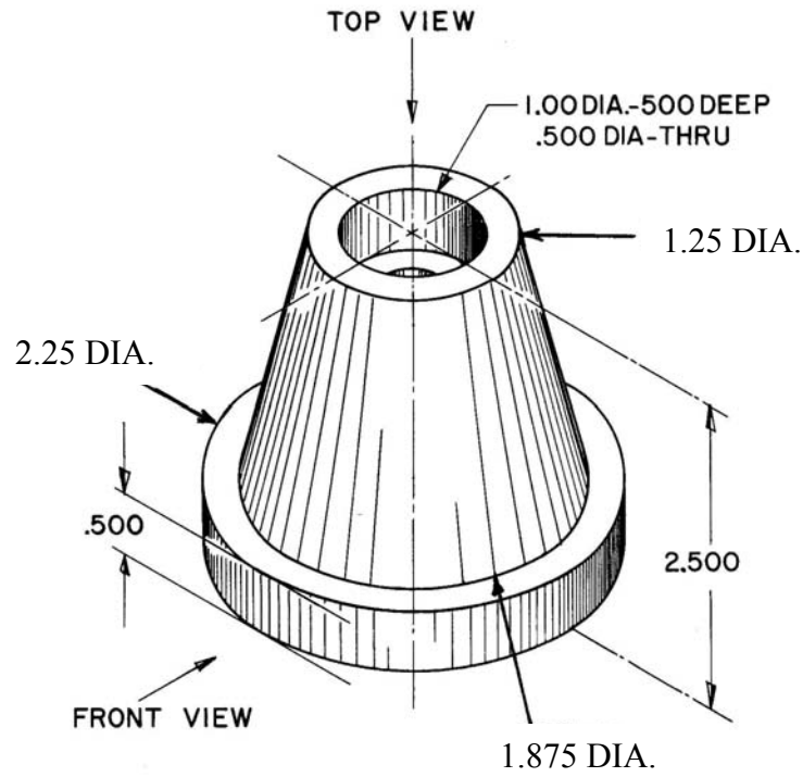
IN- 28 Tapered Support
